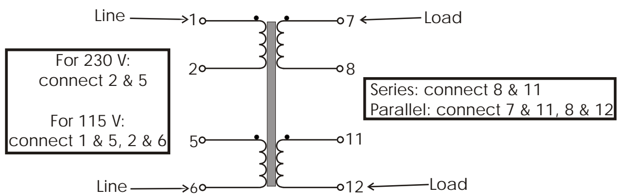
Schematic Diagram
